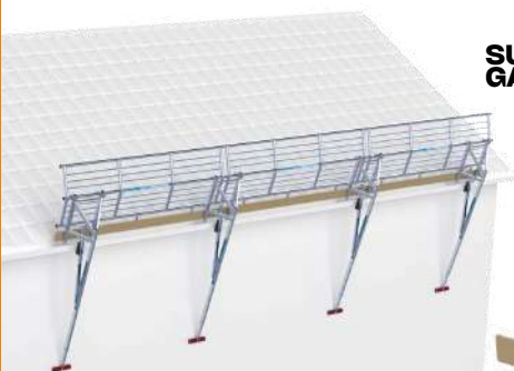
GARDE-CORPS 3000x1000mm
